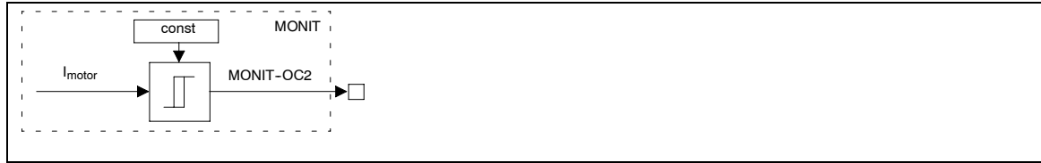
Fig. 2-148 Earth-fault monitoring (OC2)
