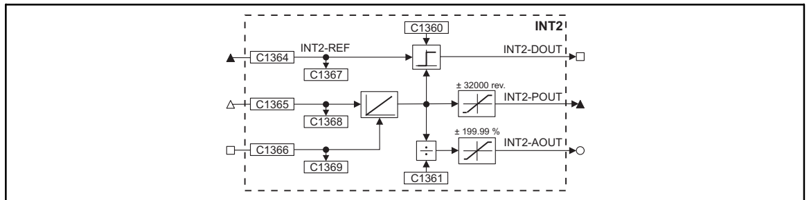
Fig. 2-90 Integrator (INT2)
