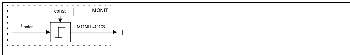
Fig. 2-149 Overload during acceleration or deceleration OC3
