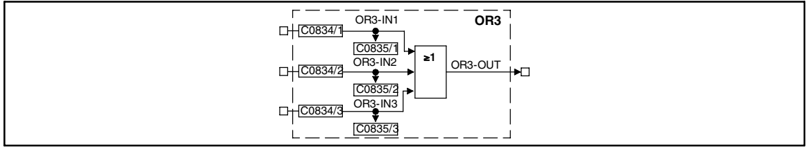
Fig. 2-116 Logic OR (OR3)
