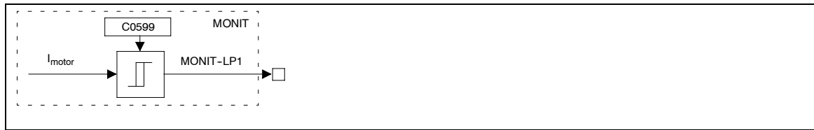
Monitoring of the motor phases (LP1)
