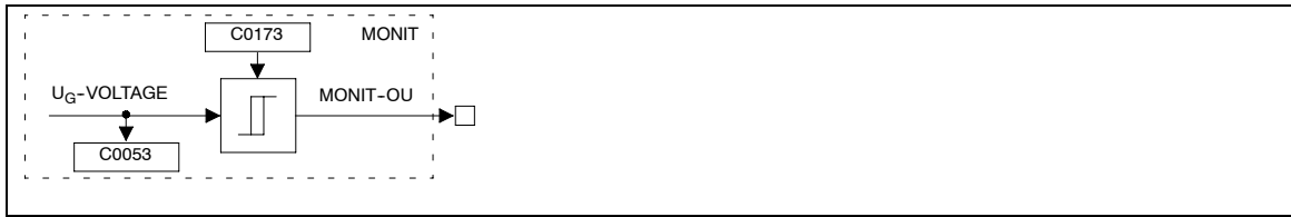
Fig. 2-157 Monitoring of overvoltage in the DC bus (OU)
