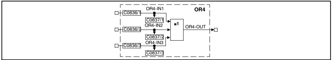
Fig. 2-117 Logic OR (OR4)
