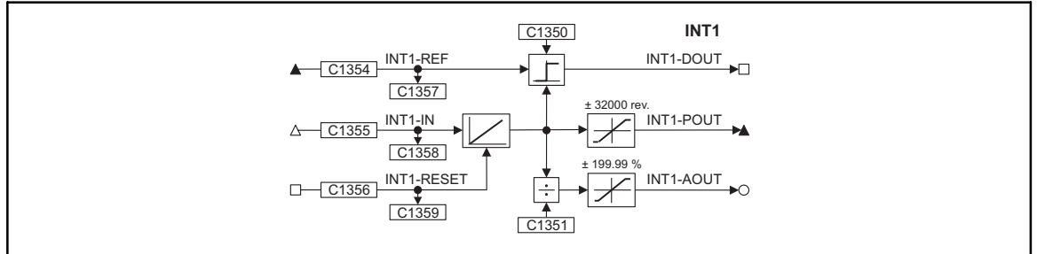
Fig. 2-89 Integrator (INT1)
