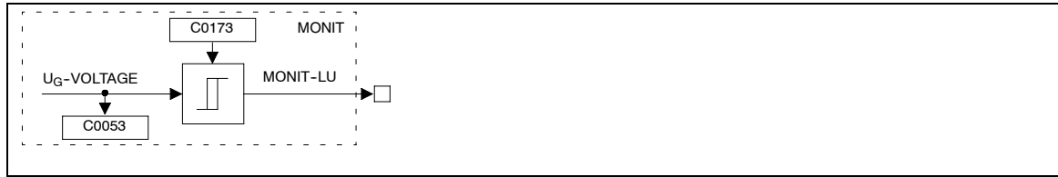
Fig. 2-156 Low voltage monitoring in the DC bus (LU)
