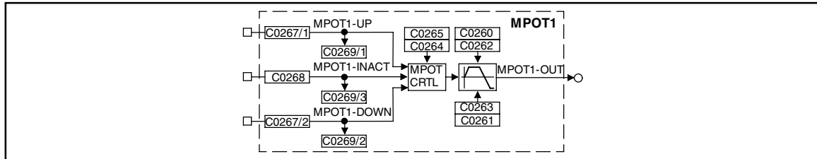
Fig. 2-101 Motor potentiometer (MPOT1)
