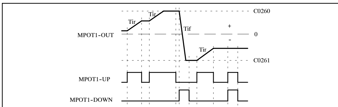
Fig. 2-102 Control signals of the motor potentiometer
