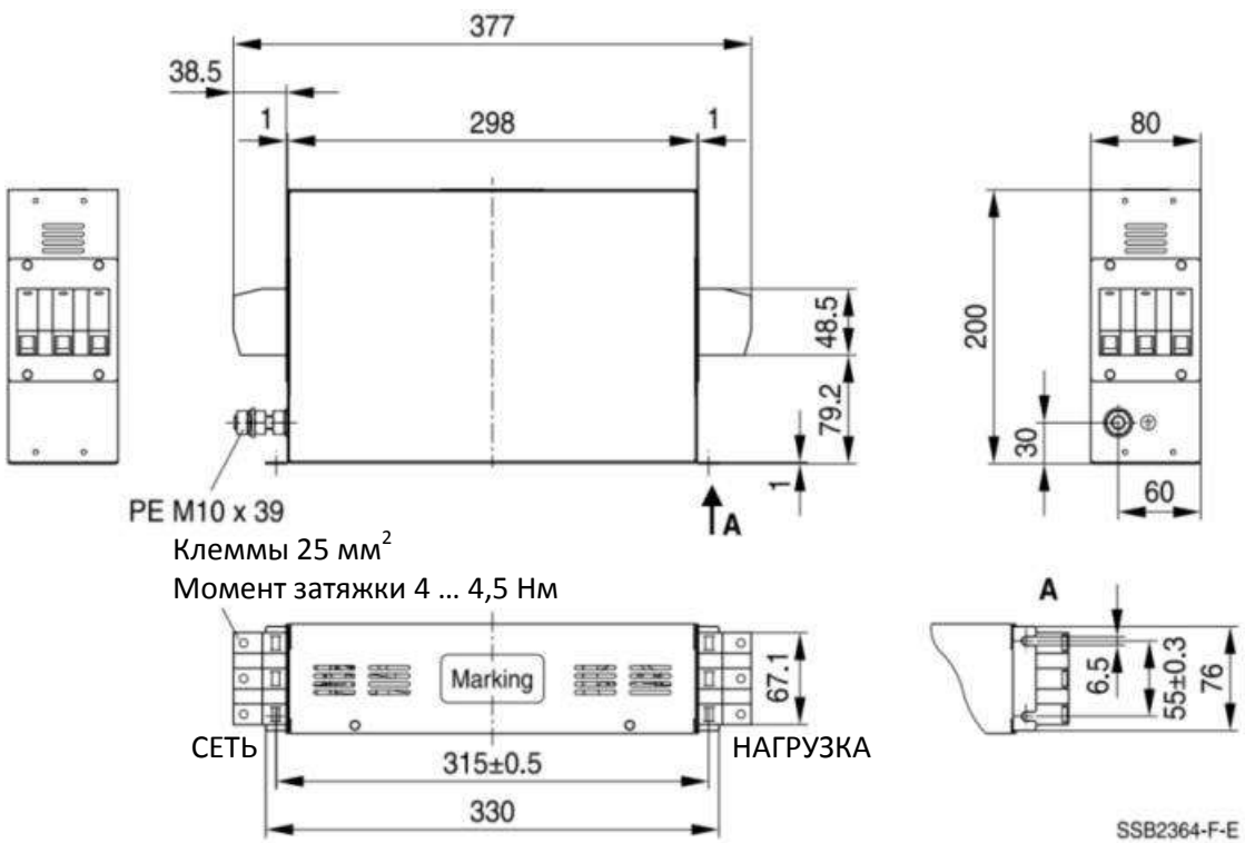
TDK B84143D0050R127 (50A)
