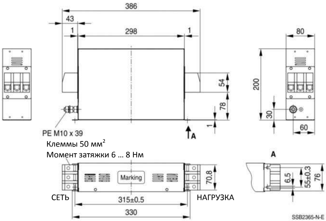
TDK B84143D0075R127 (75A), TDK B84143D0090R127 (90A)
