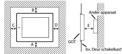
* Wanddikte: 2,0 – 4,0 mm
